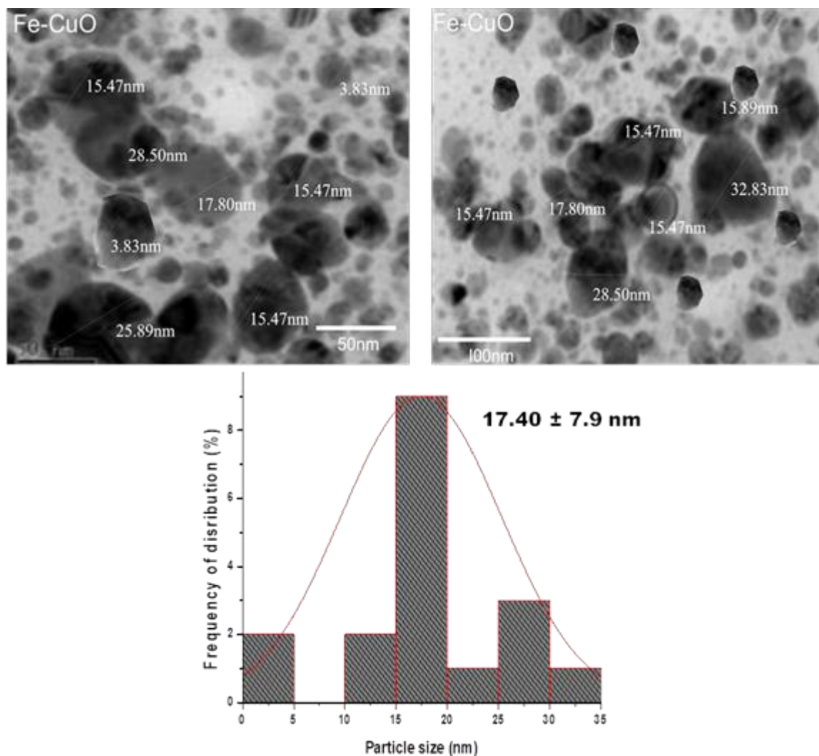
Figure 1: TEM image of the Fe-CuO Nps at different magnifications and the corresponding histogram
