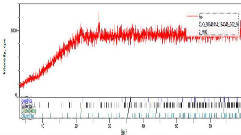
Figure 2: XRD pattern of iron-doped copper oxide nanoparticles (Fe-CuO Nps)
