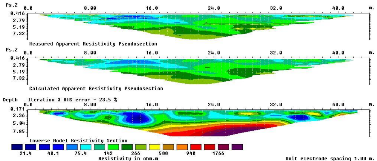
Figure 7: Resistivity distribution along profile two.
