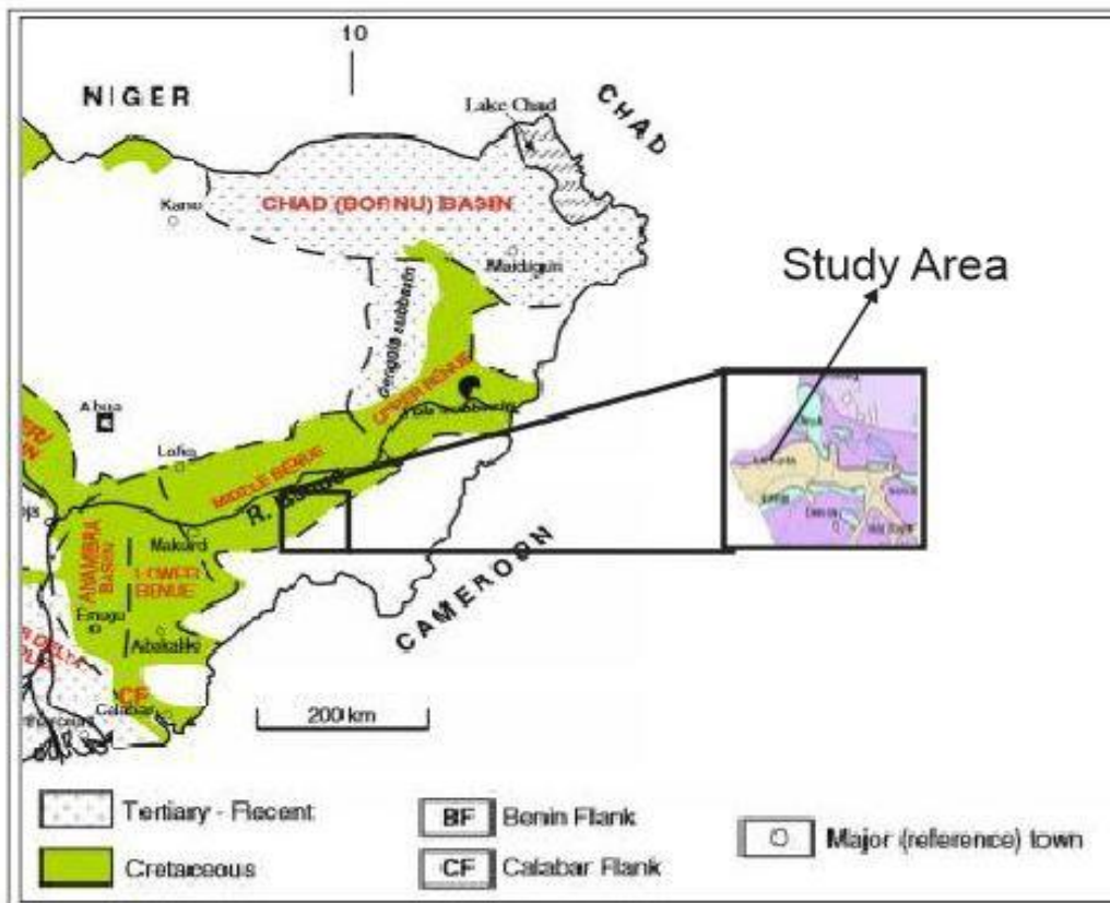
Figure 3: Geological sketch map Sedimentary Basins of Nigeria along the Study Area (modified after Obaje, 2009)
