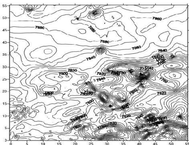
Figure 5: Aeromagnetic Map of the Study Area, contoured at 10nT
