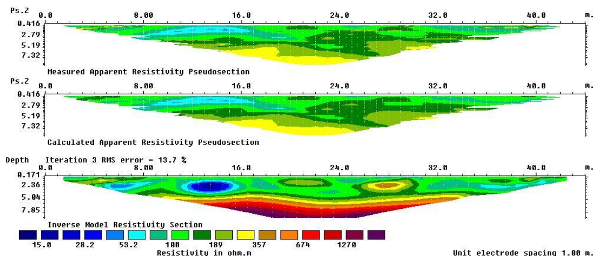
Figure 8: Resistivity distribution along profile three.
