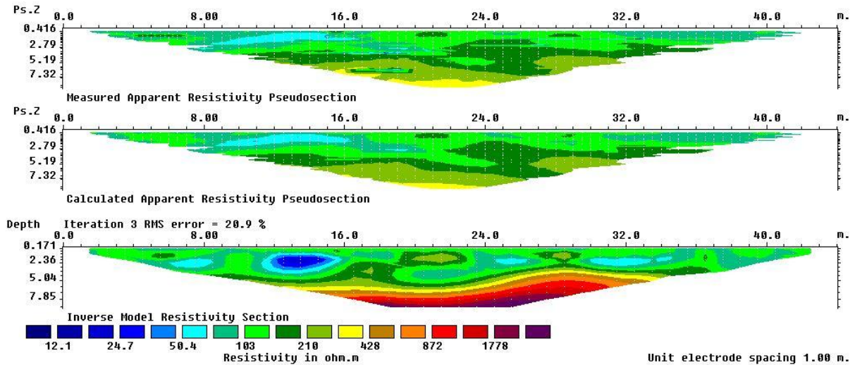
Figure 6: Resistivity distribution along profile one.
