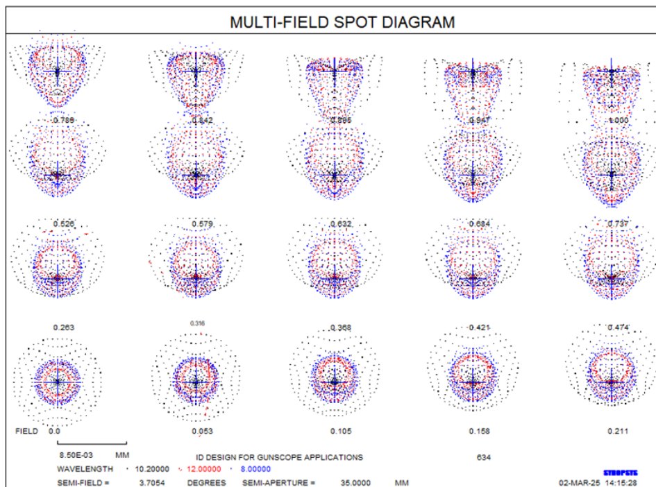
Figure 11: Multi-Field Spot Diagram on 17 \mu m pixel
