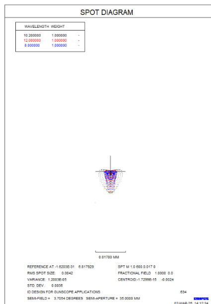
Figure-10: Spot diagram for Full FOV on 17µm
