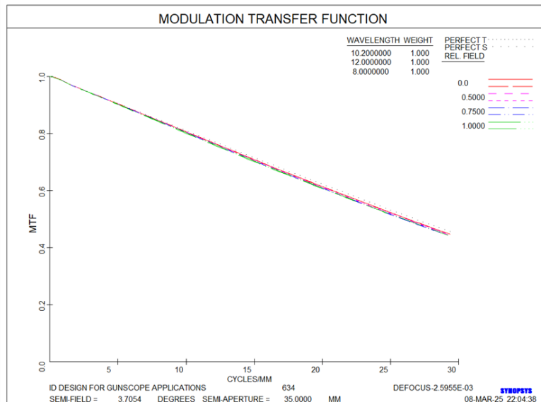
Figure-7: Polychromatic Diffraction Limited MTF at Nyquist Frequency 29.4 lp/mm
