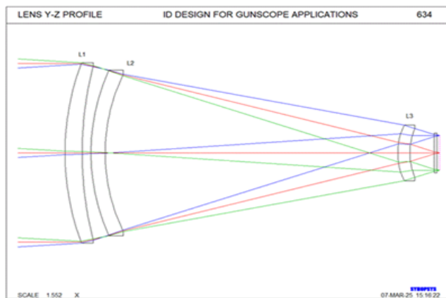
Figure 2: 2D Layout
