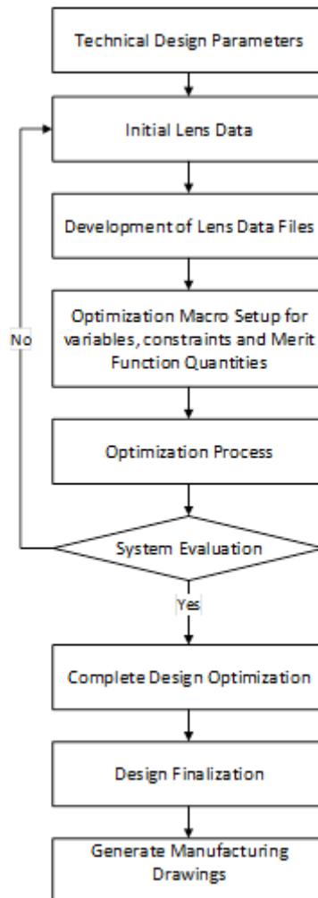
Figure-1: Gun Scope Optical Design Steps
