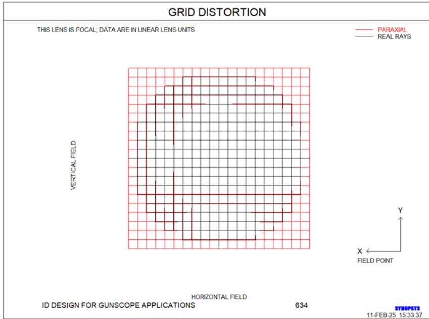
Figure 13: Grid Distortion
