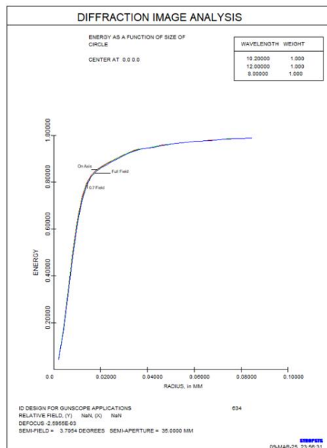
Figure 14: Encircled Energy Plot
