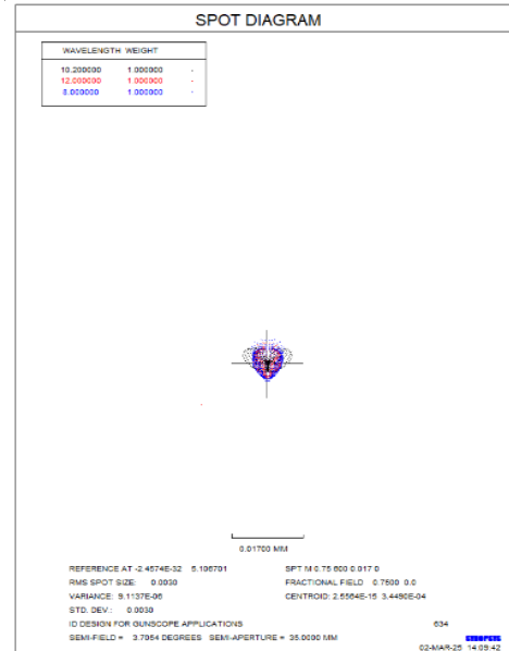
Figure 9: Spot Diagram for 0.75 FOV on 17µm
