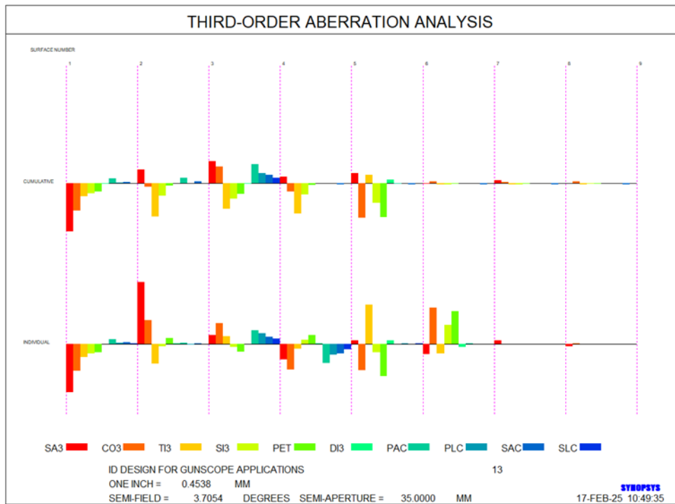
Figure-5: Third Order Aberration Analysis Graphical Representation
