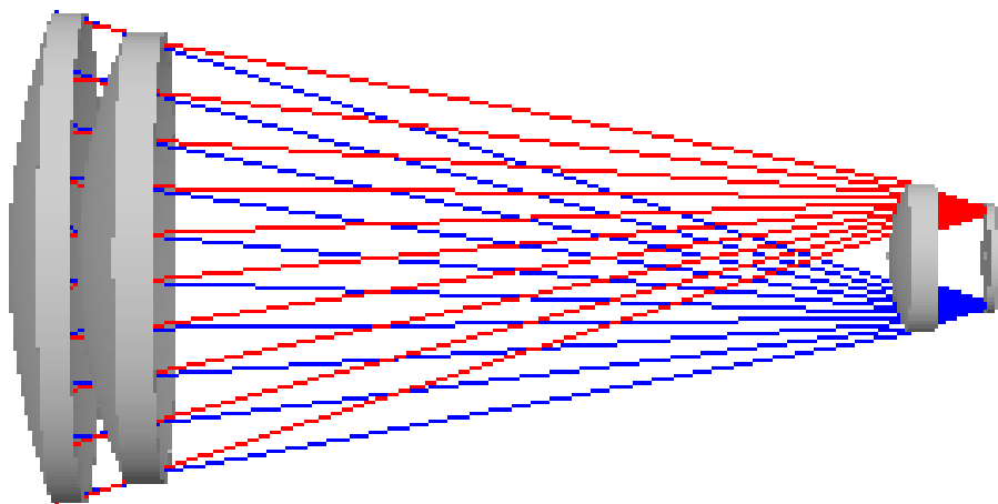
Figure 4: Shaded Model
