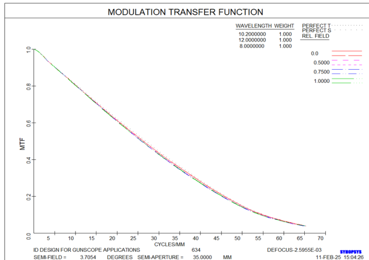
Figure-6: Polychromatic Diffraction Limited MTF at Cut off Frequency 65.3 lp/mm
