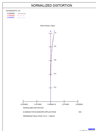
Figure 12: Normalized Distortion
