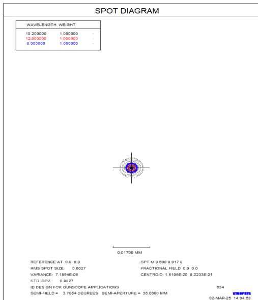
Figure 8: Spot Diagram for on axis on 17µm
