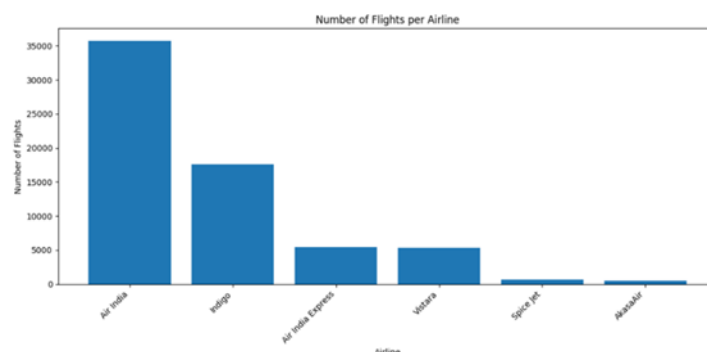
Fig.1. Number of Flights per Airline
