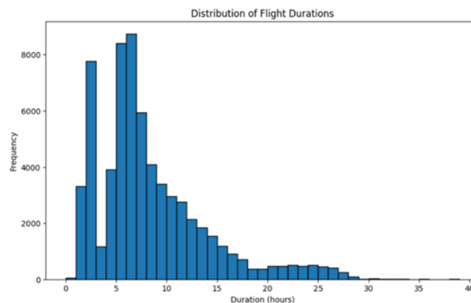
Fig.4. Distribution of Flight Durations
