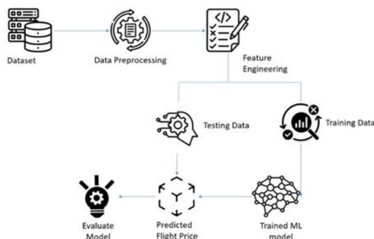
Fig.5. Architecture Diagram
