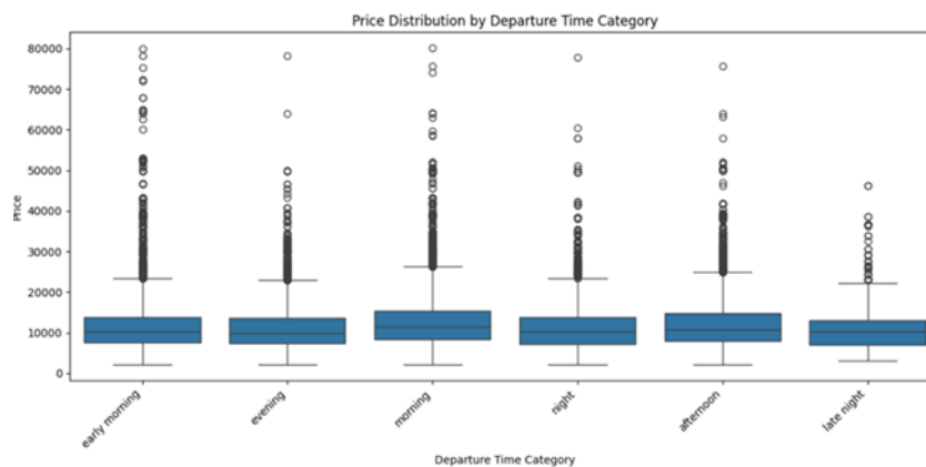
Fig.3. Price Distribution by Departure Time category
