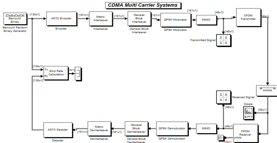
Fig. 3. simulation model of MC-CDMA
