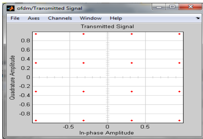
Fig. 4 Transmitted signal
