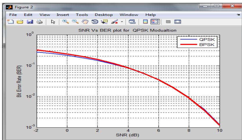
Fig. 7 BER Using one transmitting antenna and one receiving antenna for QPSK and BPSK Modulation technique.
