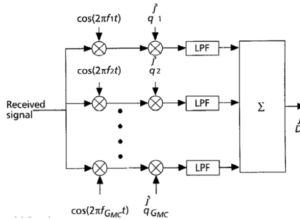
Fig. 2. MCCDMA Receiver
