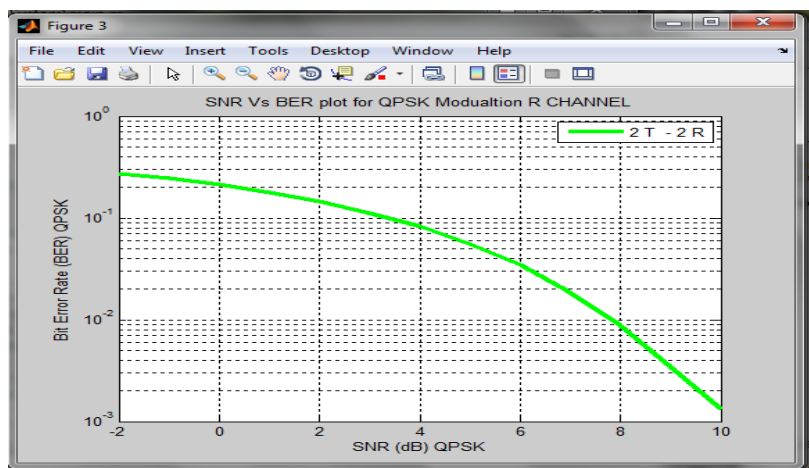
Fig 8 BER Using two transmitting antenna and two receiving antenna
