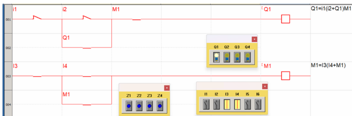
Figure 3. Ladder diagram simulation
