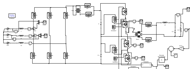
Fig14 Matlab/Simulink Model of Proposed Multilevel Full Bridge Converter with closed loop
