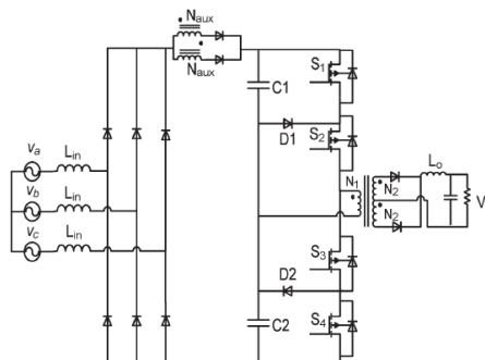
Fig.2 Newly Proposed AC/DC Single Stage Converter
