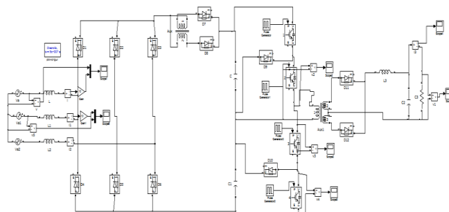
Fig. 5 Matlab/Simulink Model of Proposed Multilevel Full Bridge Converter
