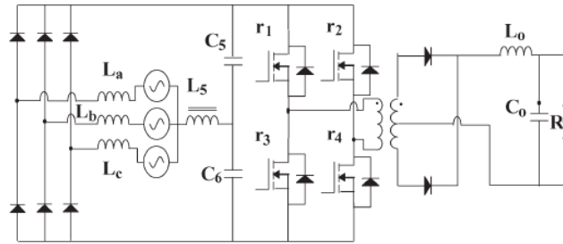
Fig.1 Previous proposed AC/DC Single Stage Converter
