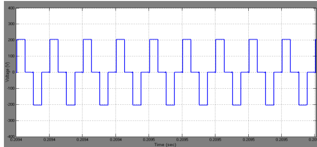
Fig.7 Voltage at Primary side Transformer
