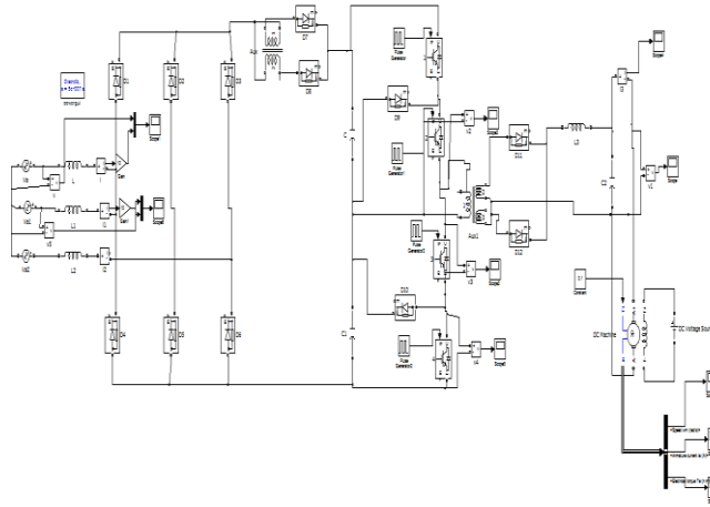
Fig. 10 Matlab/Simulink Model of Proposed Multilevel Full Bridge Converter with machine load
