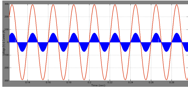
Fig. 6 Input current and voltage
