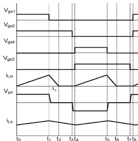
Fig. 3. Typical waveforms describing the modes of operation.
