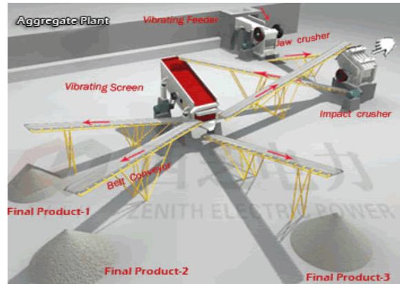
Photo2:Working Sequence of Aggregate crushing plant
