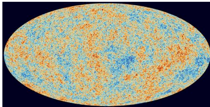
Figure 4: The Planck satellite's map of the cosmic microwave background [170]
