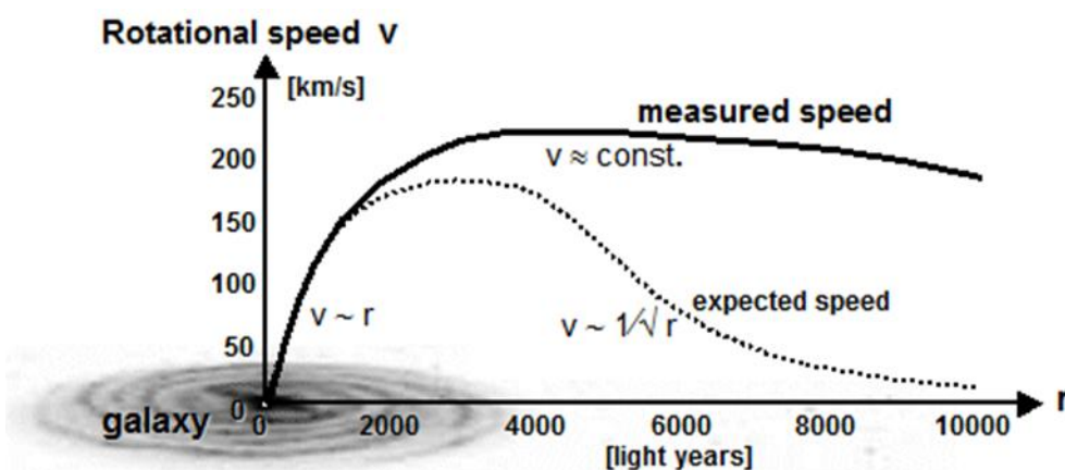
Figure 1: Typical rotation curve - dependence of the orbital velocity of matter on the distance from the center of the galaxy [96, 97].
