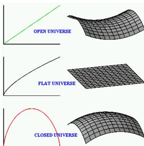
Figure 5: Large scale structure and cosmology: The ultimate destiny of the universe
