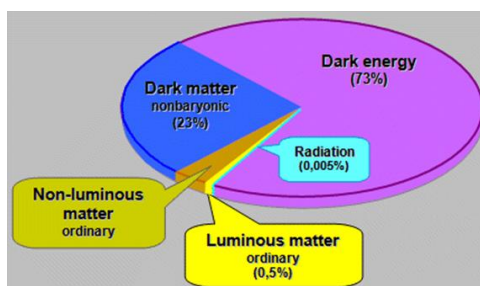
Figure 2: Basic composition of universe [161]
