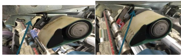
(A) (B) Fig.6. Old spring (A) and new spring (B).
