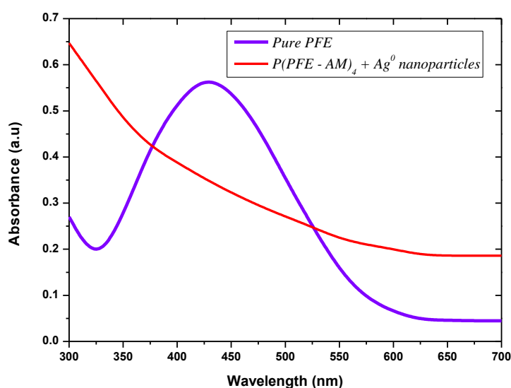
Fig.2 UV-vis of spectra of Pure PFE and \text{P(PFE-AM)}_4+\text{Ag}^0
