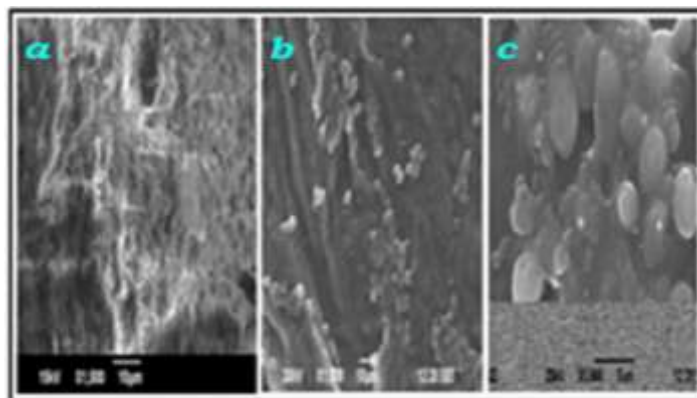
Fig.5 SEM images of: pure P(PFE-AM) 4 , P(PFE-AM) 4 +Ag + and P(PFE-AM) 4 +Ag 0 nanocomposite hydrogels
