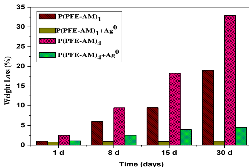
Fig.9 Biodegradation of PFE-hydrogels( P(PFE-AM)_1 and P(PFE-AM)_4 )and Ag^0 nanocomposite ( P(PFE-AM)_1+Ag^0 and P(PFE-AM)_4+Ag^0 )hydrogels by E.coli .
