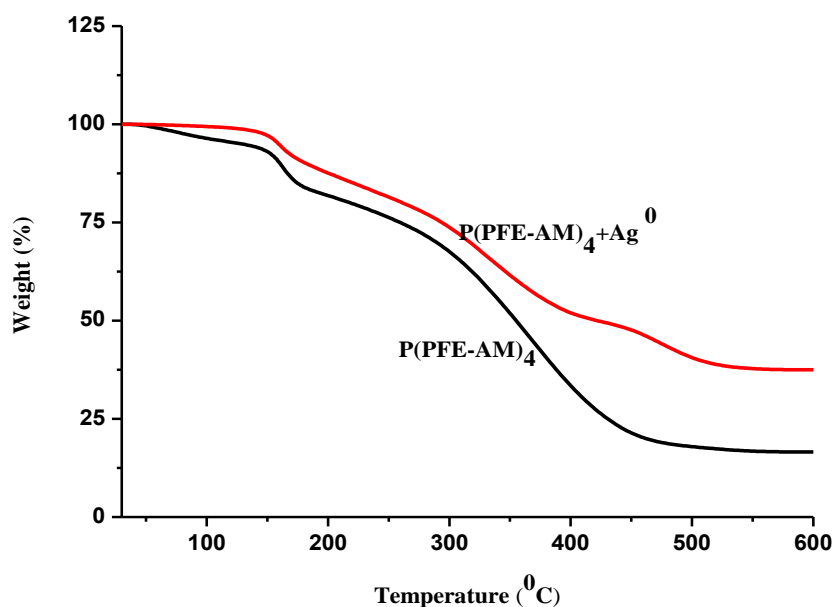
Fig.3 TGA curves of pure P(PFE-AM) 4 and P(PFE-AM) 4 +Ag 0 nanocomposite hydrogels
