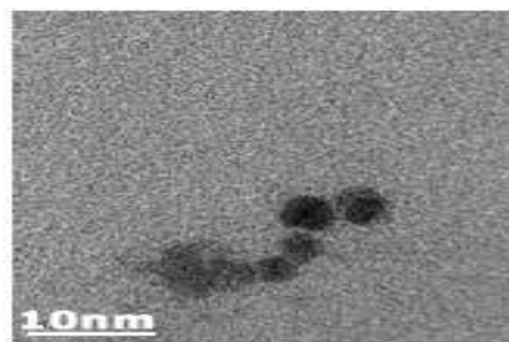
Fig.6 TEM images of P(PFE-AM) 4 +Ag 0 nanocomposite hydrogel
