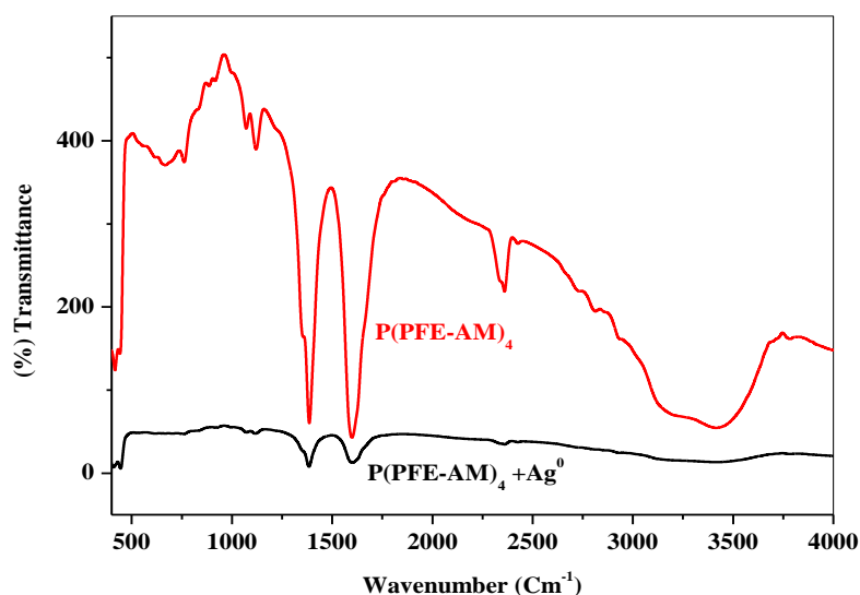
Fig.1 FTIR spectra of pure \text{P(PFE-AM)}_4 hydrogel and \text{P(PFE-AM)}_4+\text{Ag}^0 nanocomposite biodegradable hydrogels
