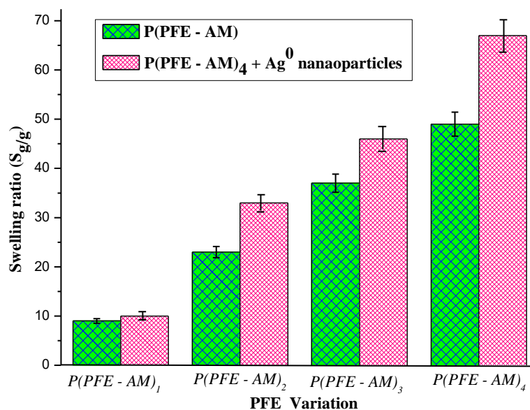
Fig.7 Swelling behaviour of P( PFE-AM) varied hydrogels and Ag 0 nanocomposite
