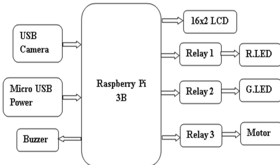
Fig.1: Block diagram of Smart rationing system by face detection
