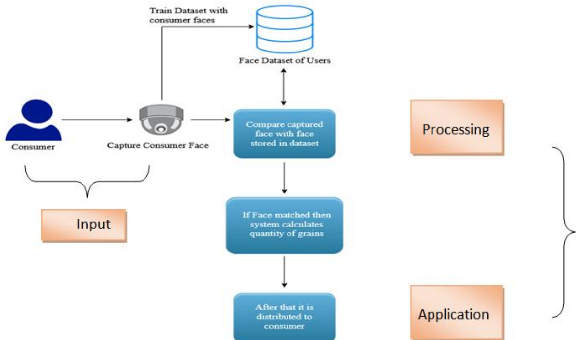
Fig 2: System Architecture
