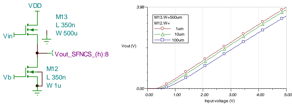
Figure 11. DC analysis of source-follower with nMOS as current-source topology for W_{13}=500\mu\text{m} , and various W_{12} . In all case V_b=2\text{V} .
