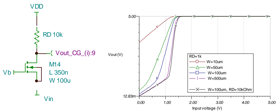
Figure 12. DC analysis of common-gate stage topology for R_D=1\text{k}\Omega and various W s and then for W_{14}=100\mu\text{m} and R_D=10\text{k}\Omega .
