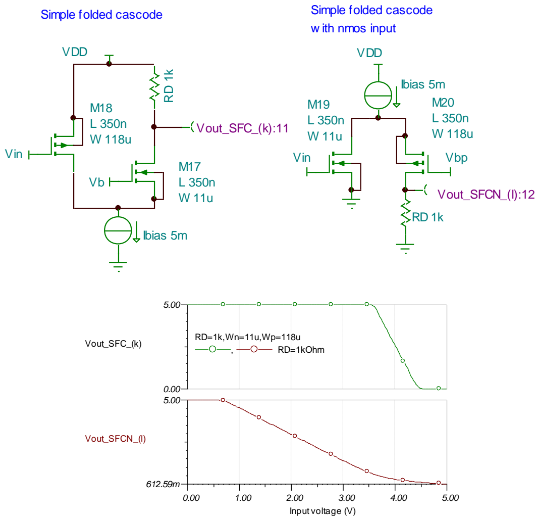
Figure 14. DC analysis for the simple-cascode stage and the simple folded-cascode stage with nMOS input, for R_D=1\text{k}\Omega , W_{nMOS}=W_{17}=W_{19}=11\mu\text{m} and W_{pMOS}=W_{18}=W_{20}=118\mu\text{m} .
