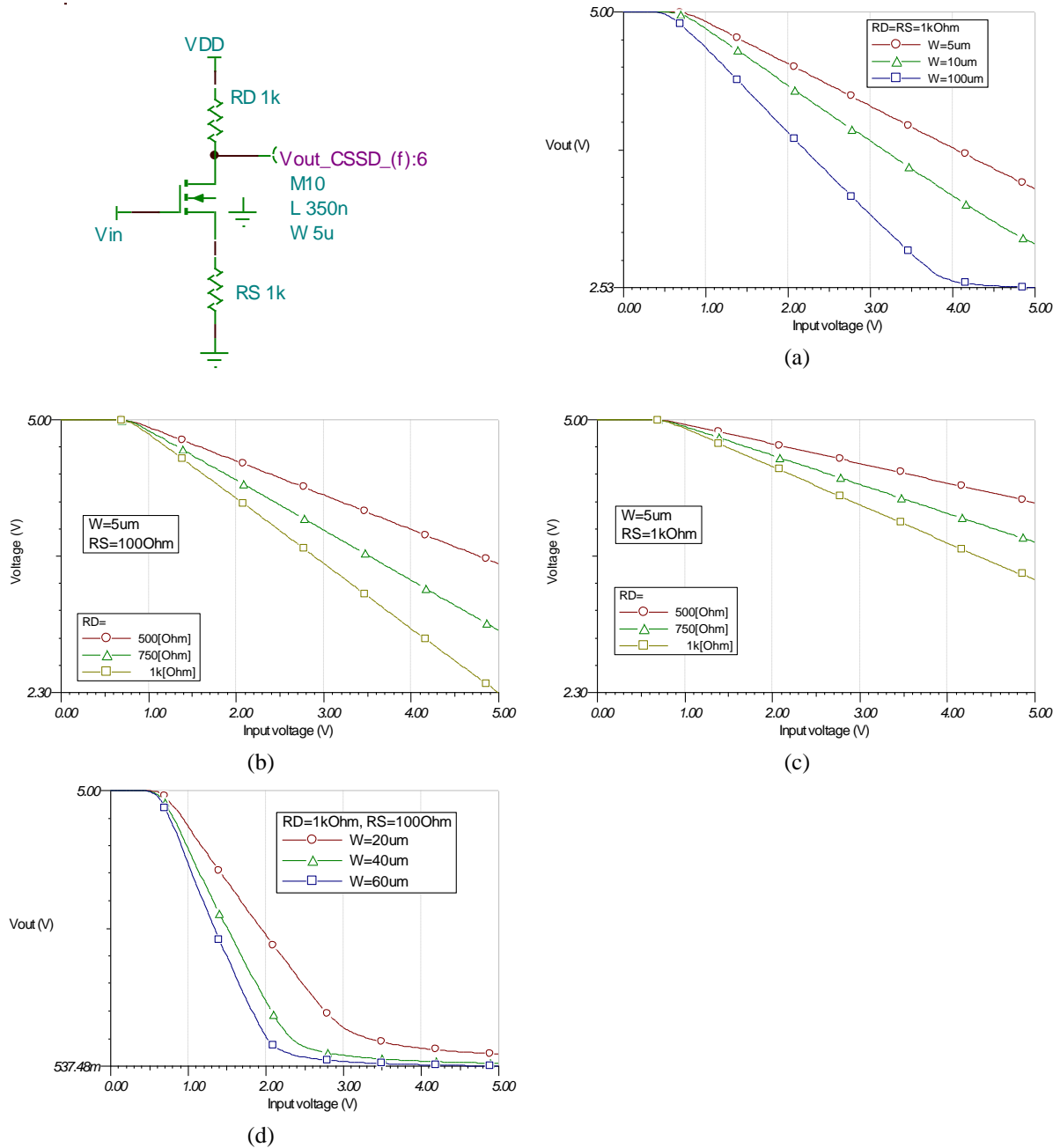
Figure 9. DC analysis of the common-source stage with source regeneration. (a) Testing various W s for R_D = R_S = 1k\Omega . (b) Testing various R_D s for W = 5\mu m and R_S = 100\Omega . (c) Testing various R_D s for W = 5\mu m and R_S = 1k\Omega . (d) Testing various W s for R_D = 1k\Omega and R_S = 100\Omega .
