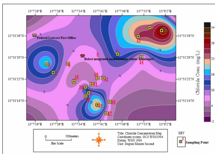
Figure 11: Map showing Concentration of Chloride in the study area
