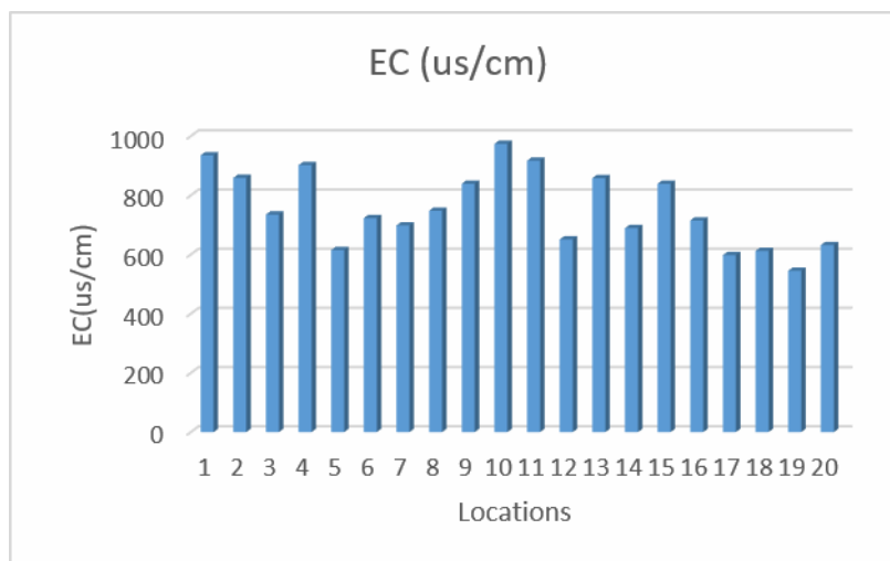
Figure 6: Histogram showing EC variations
