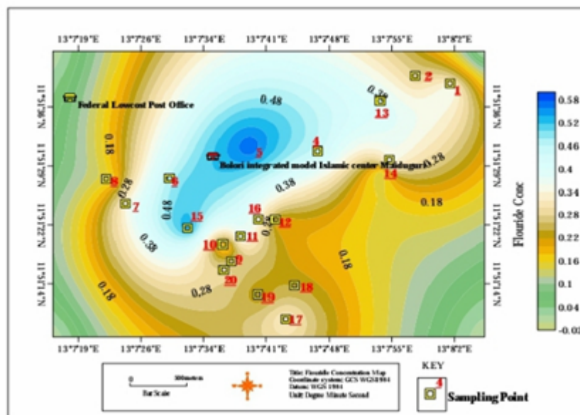
Figure 8: Map showing Concentration of Fluoride in the study area
