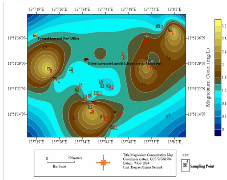
Figure 9: Map showing Concentration of Magnesium in the study area
