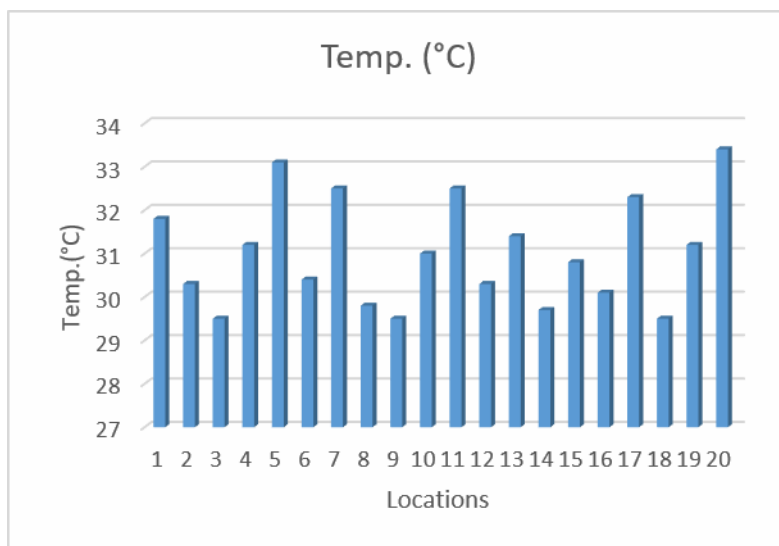
Figure 7: Histogram showing Temperature variations
