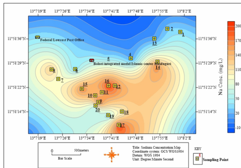
Figure 10: Map showing Concentration of Sodium in the study area
