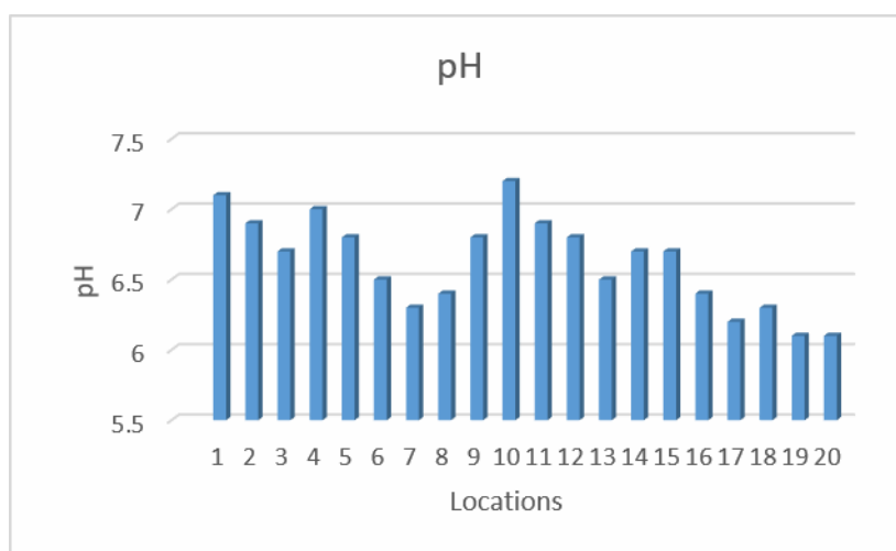
Figure 4: Histogram showing pH variations
