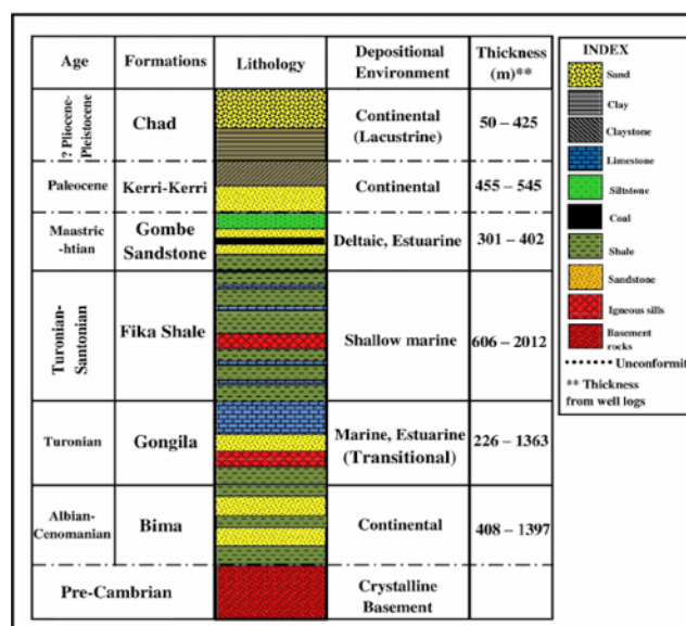
Figure 2: Stratigraphy of the Bornu Basin, Northeastern Nigeria (after Okosun 1995; Avbovbo et al. 1986; Carter et al. 1963)
