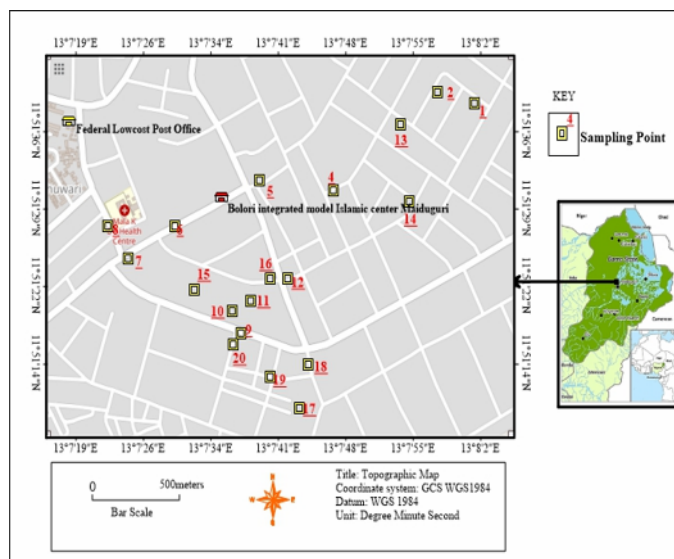
Figure 3: Topography of the study area showing sample locations
