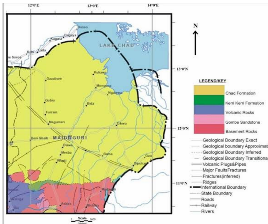
Figure 1: Geology of the Bornu basin (NGSA, 2006)
