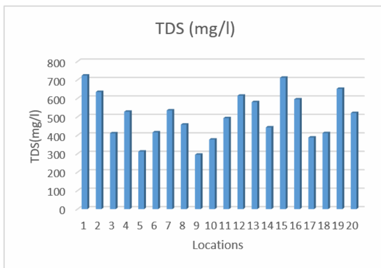
Figure 5: Histogram showing TDS variations within the study area
