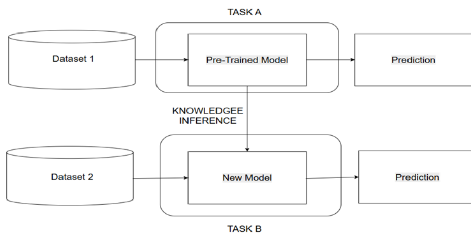
Figure 2: Transfer Learning
