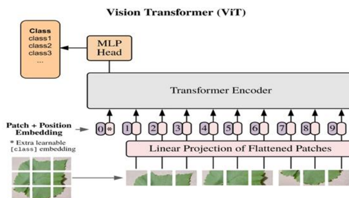
Figure 3: Vision Transformers Architecture[17]
