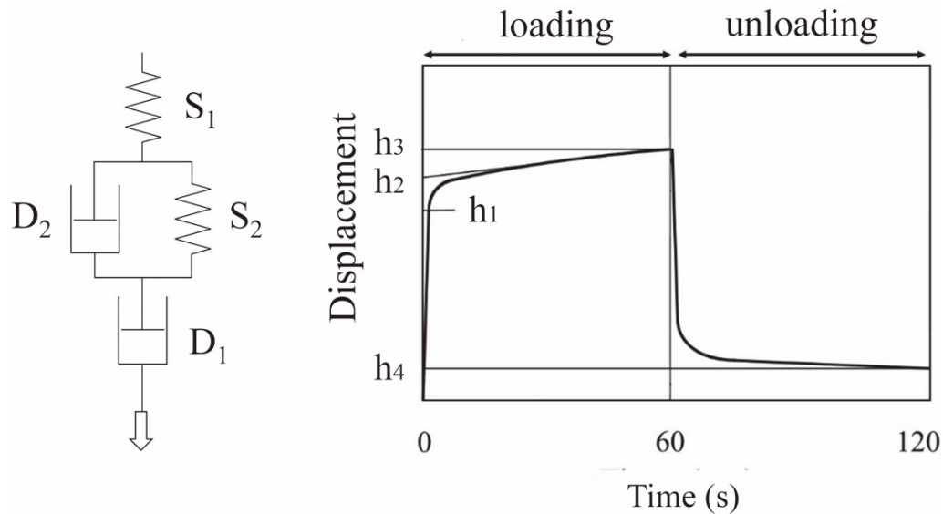
FIGURE 11- CIRCUIT AND GRAPHICAL REPRESENTATION OF RHEOMETER
