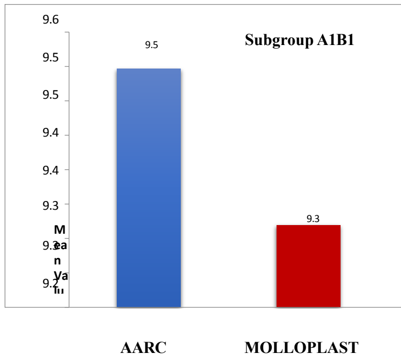
Graph II
