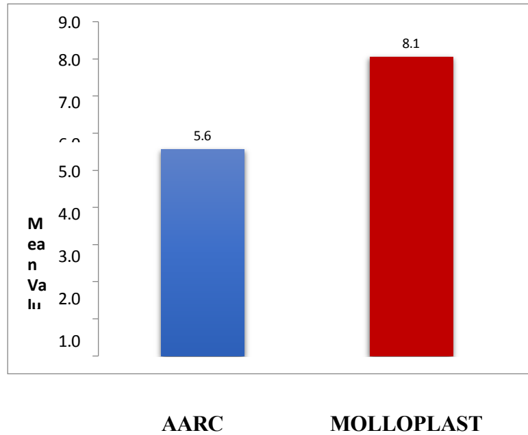
Subgroup A3B3
