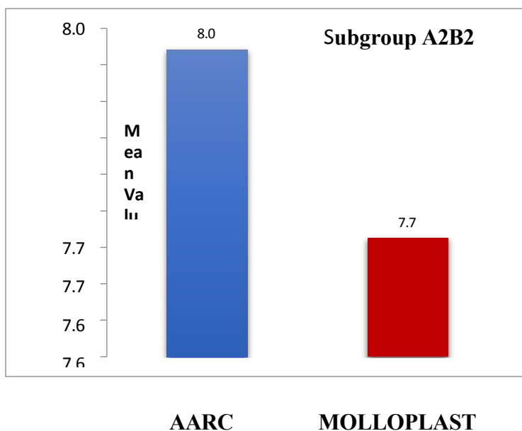
Graph III
