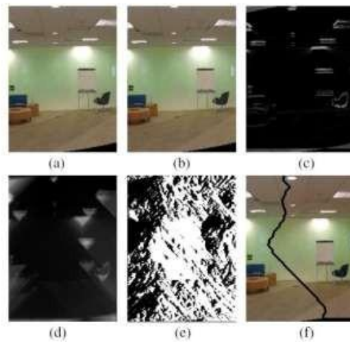
Fig -5: Process of finding the optimal seam with dynamic programming optimization.
