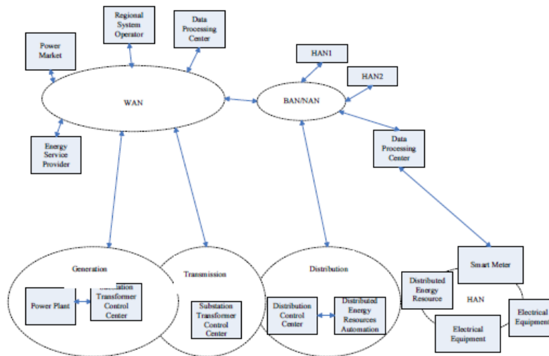
Fig.2.The Smart Grid Communication Infrastructure [3].
