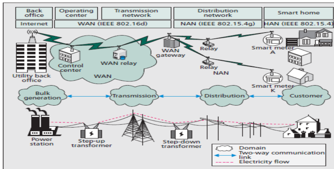
Fig.1. A conceptual model for deployment of smart electricity grid [2].
