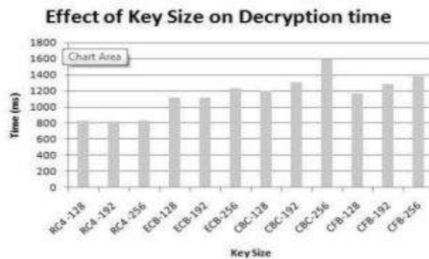
Graph.4: Decryption time of RC4 and AES (with Key sizes)
