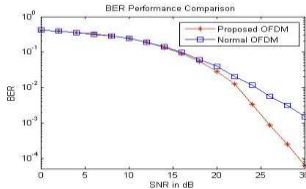
Fig.5 BER vs SNR curves comparing the performance of the proposed scheme with a conventional OFDM scheme without employing the diversity.
