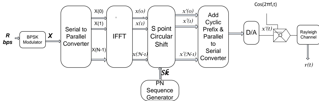
Fig.2 Scheme showing OFDM transmitter with subcarrier diversity
