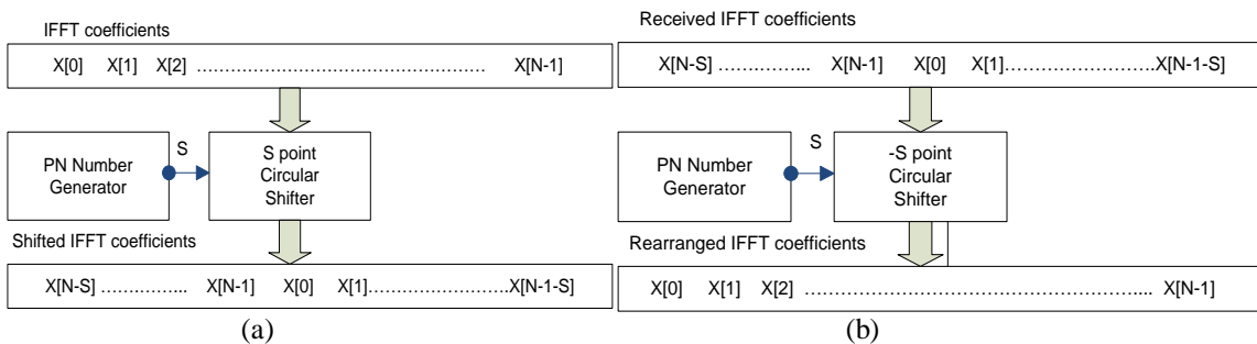
Fig.4 The detailed description of coefficient shift scheme (a) Scheme showing the S point IFFT Co-efficient shift (b) Scheme showing rearrangement of coefficients by -S point shift
