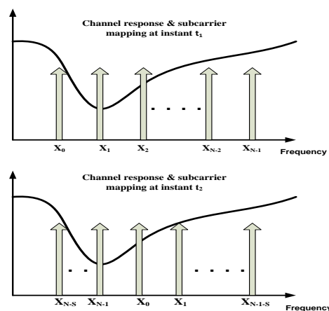
Fig. 1. Illustration of channel response and its effect on subcarrier mapping. As we can see at time instant t_1 subcarrier X_1 experiences deep fade but X_{N-1} does not. At t_2 , it's vice versa
