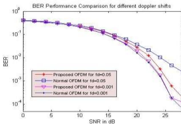
Fig.6 BER performance comparison at two different Doppler shifts, 'fd'. Note the similar performance at lower Doppler shifts but improvement is found for higher shifts.
