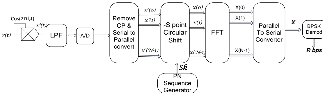
Fig.3 Scheme showing OFDM receiver with reverse shift
