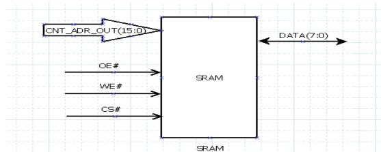
Figure2: Asynchronous SRAM
