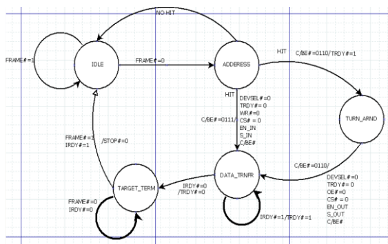
Figure4: Target State machine
