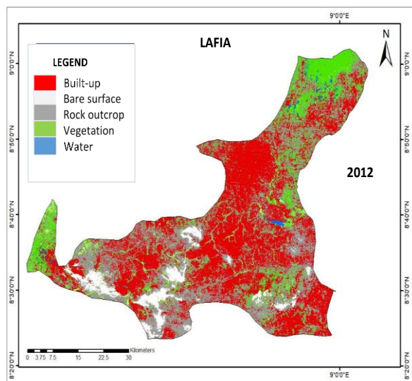
Figure 5: 2012 LULC of Lafia
