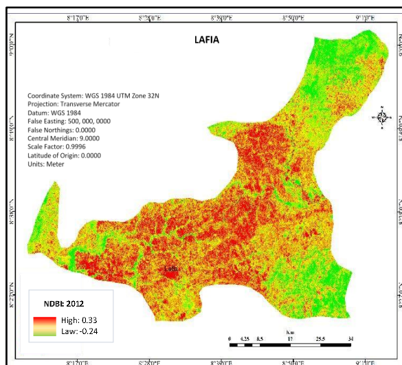
Figure 8: 2012 NDBI of Lafia
