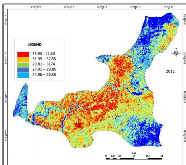
Figure 11: 2012 LST of Lafia
