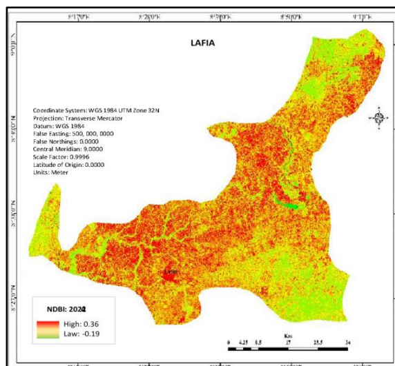
Figure 9: 2024 NDBI of Lafia
