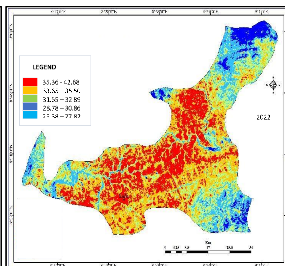
Figure 12: 2024 LST of the Lafia
