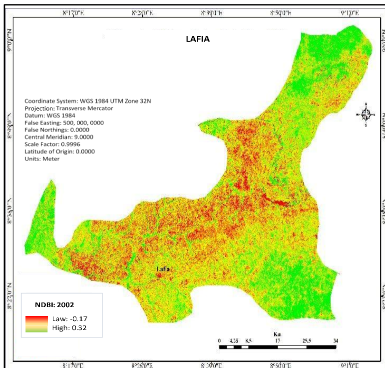
Figure 7: NDBI of Lafia 2002
