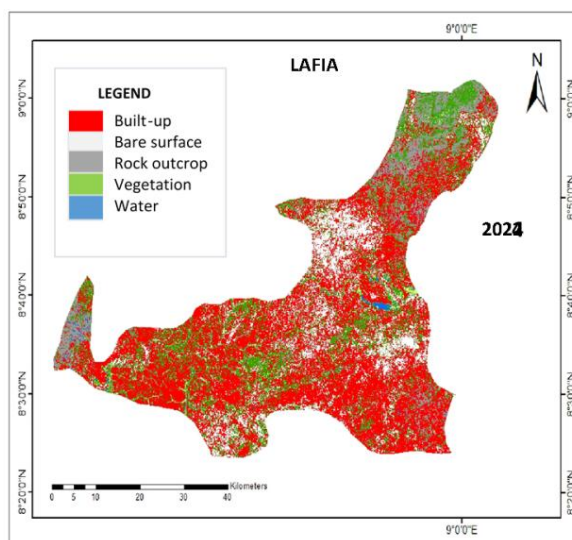
Figure 6: 2024 LULC of Lafia
