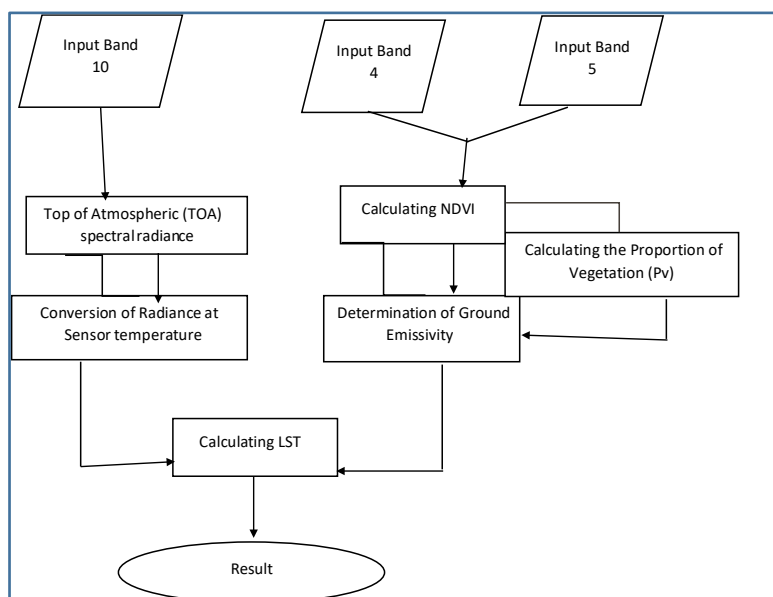
Figure 3. Algorithm for SUHI Evaluation And Assessment
