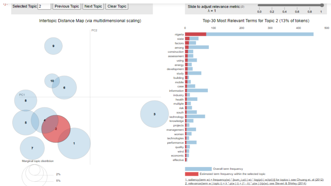
Figure 4.2: The layout of LDAvis, with the global topic view on the left, and the term bar charts (with Topic 2 selected) on the right. Linked selections allow users to reveal aspects of the topic-term relationships compactly
