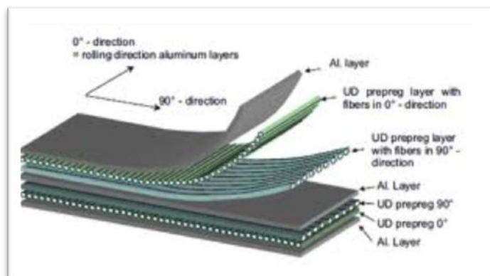
Fig.1 Fiber Metal Laminate
