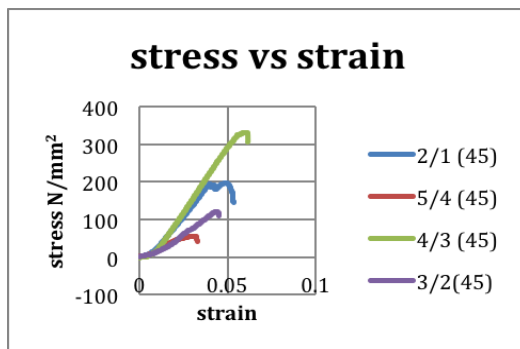
Fig. 15 stress vs strain for tensile test
