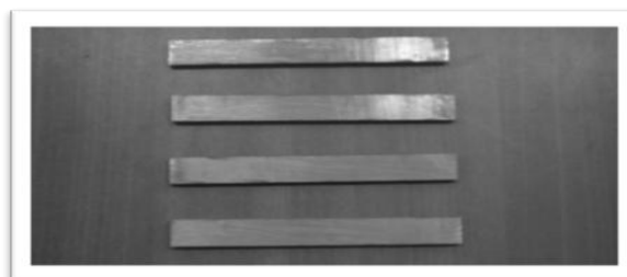
Fig. 11 specimen before flexural test
