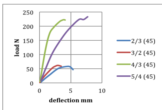
Fig. 16 load vs deflection for flexural test
