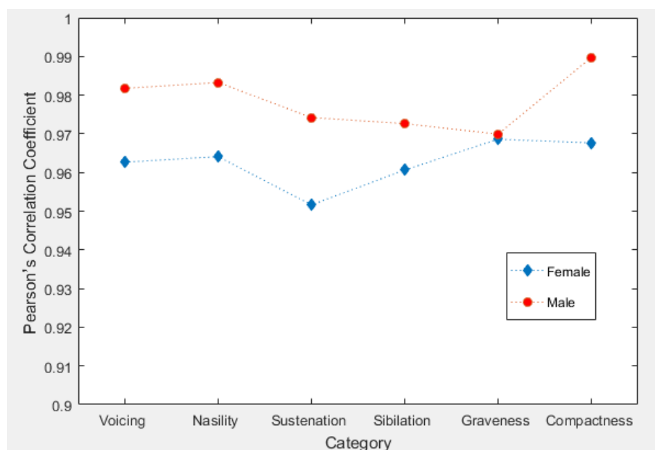
Figure6: The Average Pearson's Correlation Coefficient between the synthesized speech signal and the recorded signals in each category.
