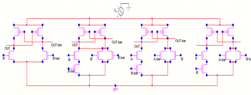
Fig. 9: ECRL 2x2 bit Square
