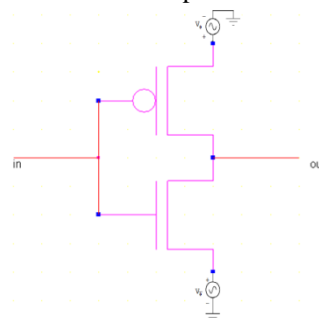
Fig. 5: Adiabatic inverter
