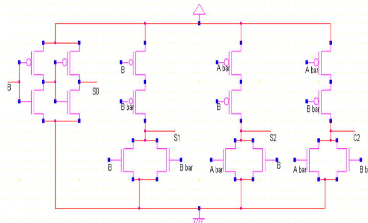
Fig. 4: CMOS 2x2 bit Square
