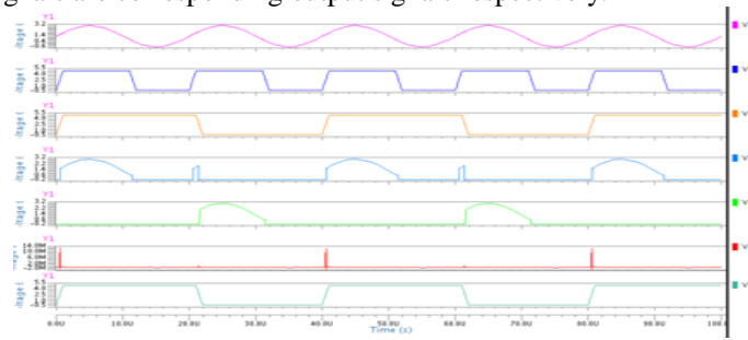
Fig. 17: Simulated waveforms of ECRL 2x2 bit Square
