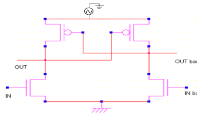
Fig. 8: ECRL inverter
