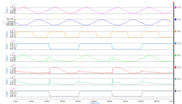
Fig. 19: Simulated waveforms of 2PASCL 2x2 bit Square
