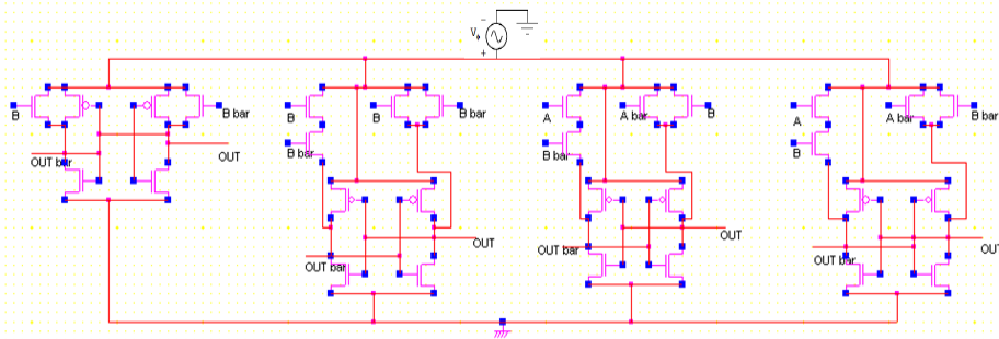
Fig. 11: PFAL 2x2 bit Square
