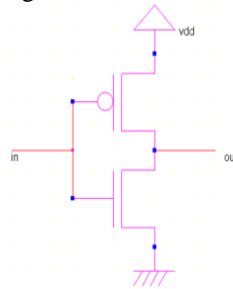
Fig. 1: CMOS inverter
