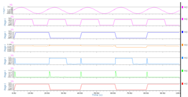
Fig. 18: Simulated waveforms of PFAL 2x2 bit Square
