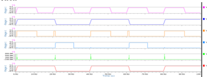
Fig. 16: Simulated waveforms CMOS 2x2 bit Square
