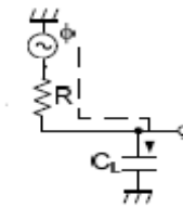
Fig. 6: Equivalent circuit for charging process in adiabatic inverter
