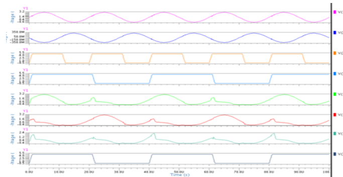
Fig. 20: Simulated waveforms of PFAL&2PASCL 2x2 bit Square
